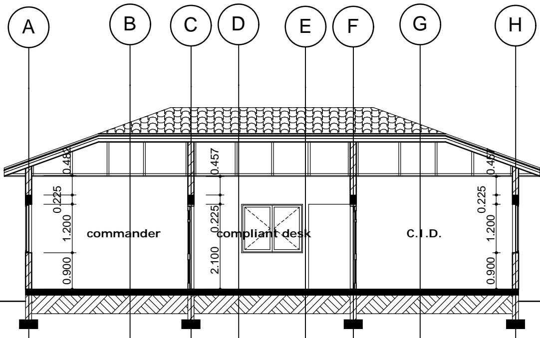
SECTION 01-01
