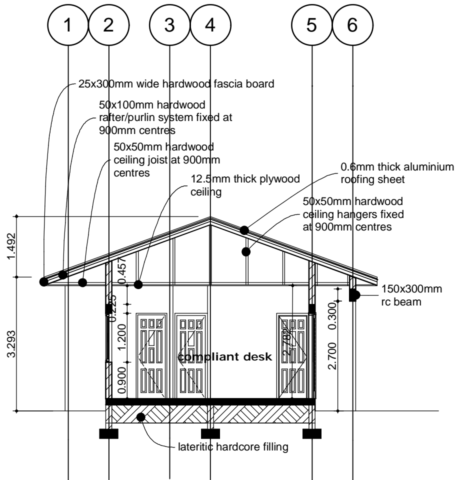
SECTION 01-01
